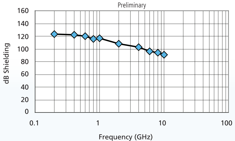
SNL70-HXP Shielding Effectiveness (dB)
